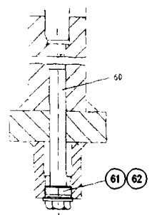
support guide of blade carrier
