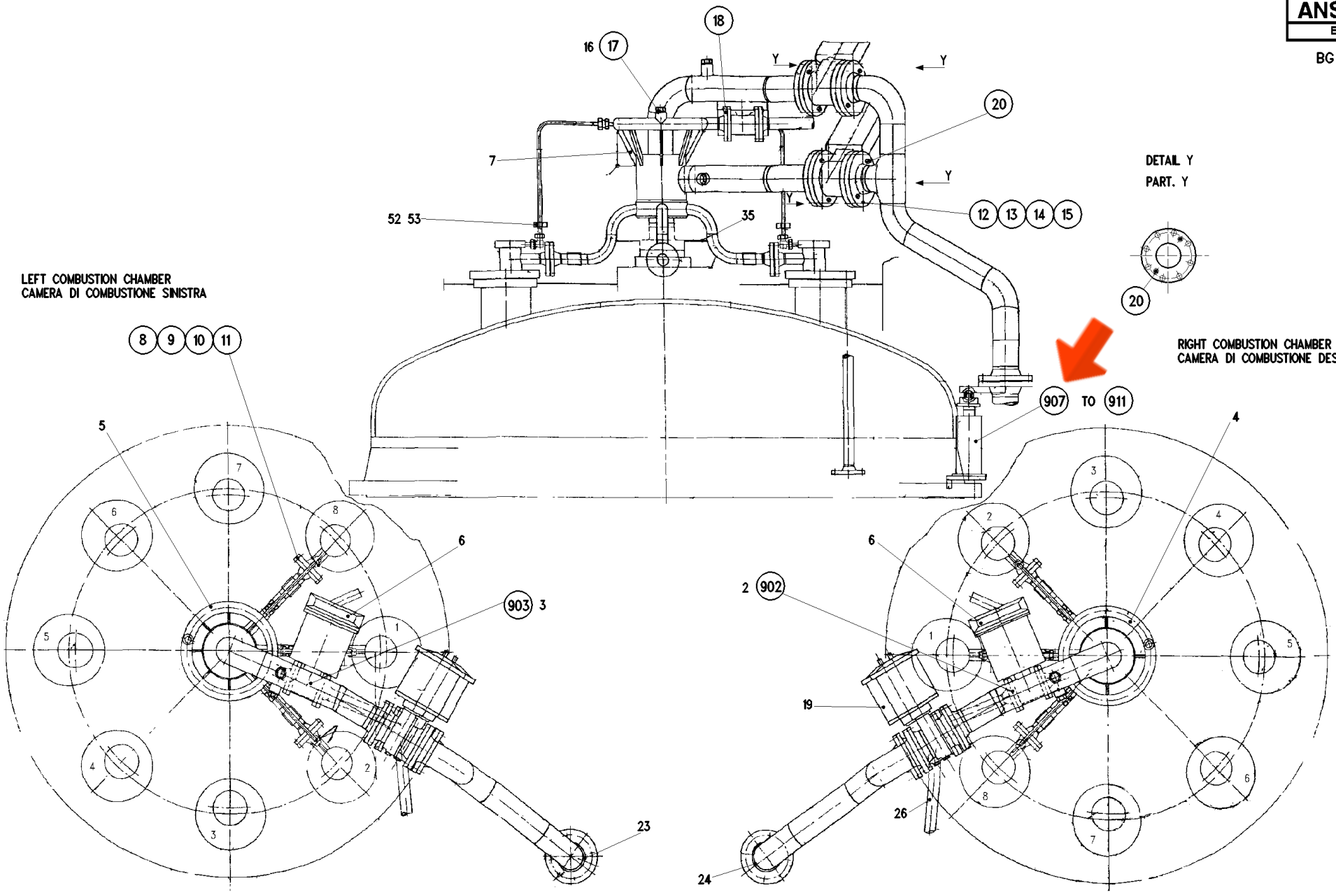
FUEL GAS PIPING AT COMBUSTION CHAMBER
