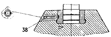
SECTION F-F
