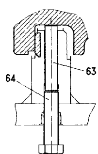
SECTION G-G
